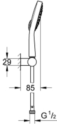
27 741 000 Power&Soul Cosmopolitan 130 Wall Holder Set +4 sprays
