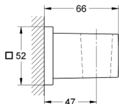
27 693 000 Euphoria Cube Wall hand Shower holder
