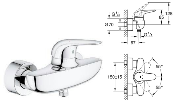
23 722 003 — 23 722 LS3 Single-lever shower mixer 1/2
