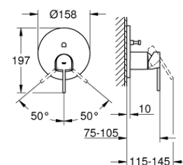
24 060 003 Single-lever mixer with 2-way diverter
