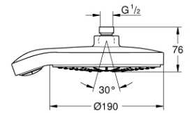
27 765 000 Power&Soul Cosmopolitan 190 Head shower +4 sprays
