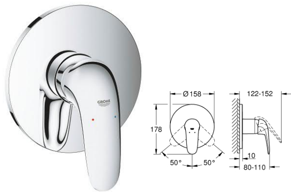
24 046 003 — 24 046 LS3 Single-lever shower mixer trim
