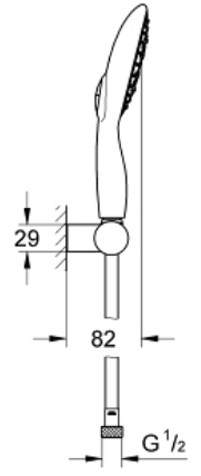
27 742 000 Power&Soul Cosmopolitan 130 Wall Holder Set +4 sprays
