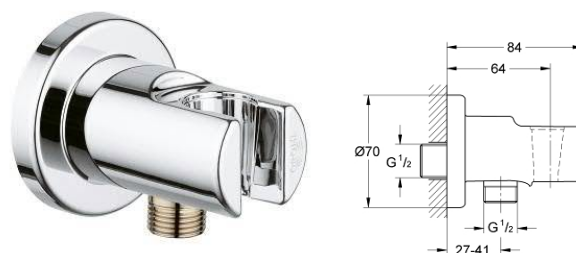
28 628 000 Relexa Shower outlet elbow, 1/2
