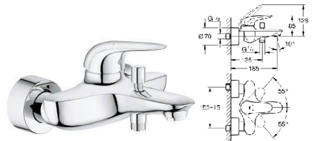
23 726 LS3 Single-lever bath mixer 1/2
