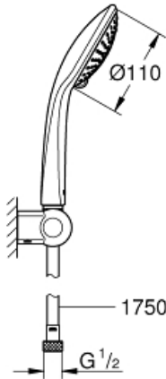
27 355 000 Euphoria 110 Champagne Wall holder set 3 sprays
