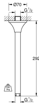
27 982 000 RAINSHOWER GRANDERA SHOWER Arm ceiling 292 mm
