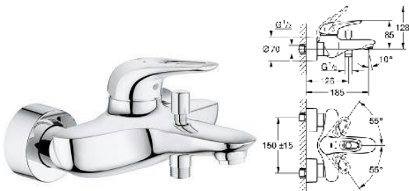
33 591 003 — 33 591 LS3 Single-lever bath/shower mixer 1/2
