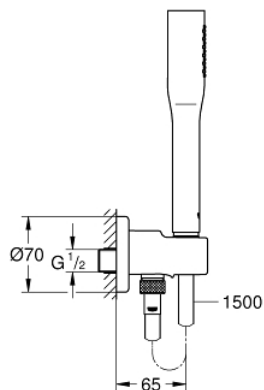
26 404 000 EUPHORIA Cosmopolitan Stick Wall Holder set 1 spray
