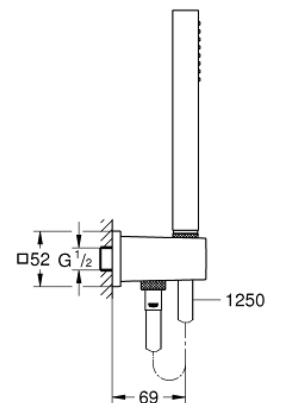
26 405 000 Euphoria Cube Stick Wall holder set 1 spray
