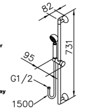
7903-9T-80CP Slide Bar Set W / Hand Shower W / Hose 150cm
