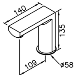
6790-N0-80CP Tip-Touch Basin Faucet (Cold Only)
