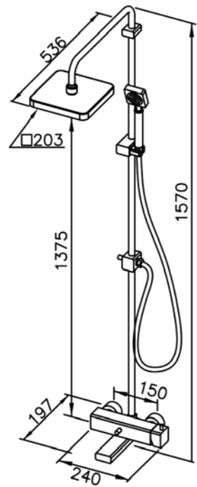
6909-BD-80CP Bath / Rainshower System
