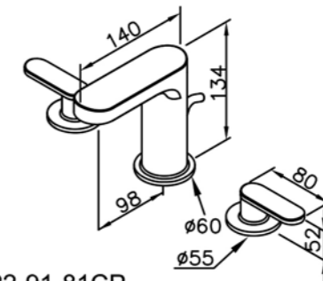
6922-91-81CP Two-Handle Lavatory Faucet W / Lift Rod W / Angle-Adjusted Aerator
