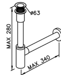
6502-N4-81CP Turn-Over W / Tail Tube W / T-Trap(6502-T1-80CP)
