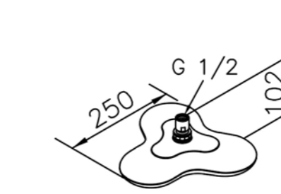
Wall-Mounted Showerhead 6903-AB-8207 Center Spray / Whole Spray
