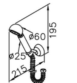
6903-9S-82CW Hand Shower W / Hose 150cm W / Wall Bracket
