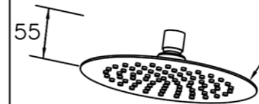
6770-A1-80S1 200mm Showerhead
