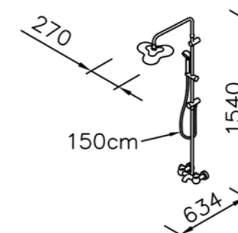
Bath / Rainshower System 6903-BD-82CP Center Spray / Whole Spray
