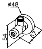
6874-Y7-80CP Angle Stop 1/2G
