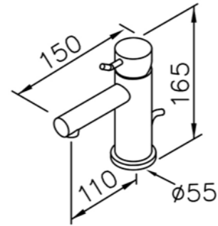
6768-90-81CP Basin Faucet W / Lift Rod
