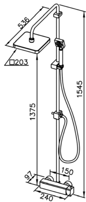
6909-BF-80CP Rainshower System
