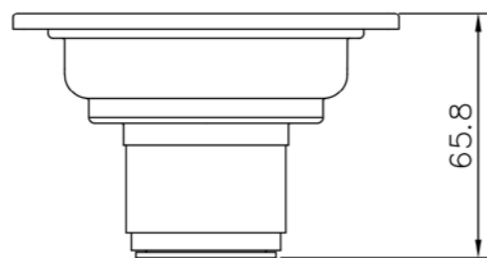
Floor Drain 100*100 mm 0305-19-79S1
