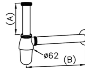
Bottle-Trap 6512-BT-80CP A:108 B:210(mm) 6512-BT-81CP A:108 B:420(mm) 6512-BL-80CP A:185 B:210(mm) 6512-BL-81CP A:185 B:420(mm)
