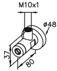
6874-Y0-80CP M10 (F) Outlet
