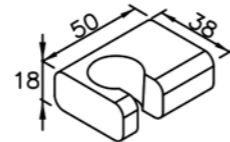
6909-9C-80CP Wall Bracket(Brass)
