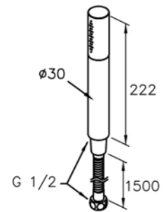
6757-9S-81CP Hand Shower W / Hose 150cm
