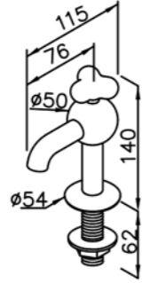
Skip Tap 6903-9A-80CP
