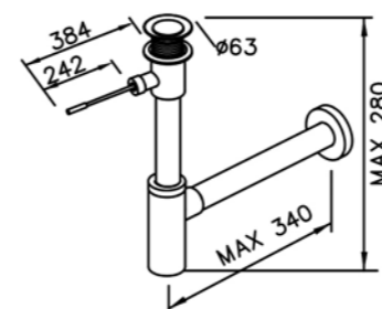
6502-N2-81CP Hand-Drive W / Tail Tube W / T-Trap(6502-T1-80CP)
