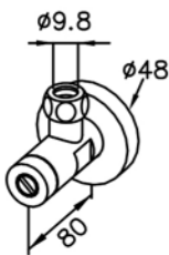
6874-Y8-81CP 1/2" IPS x 3/8" O.D.
