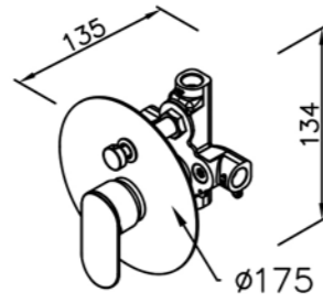
Concealed Mixer Valve W / Diverter & Check Valve W / O Inlet Stop Version 6923-XX-80CP (4~6kg/cm 2 )
