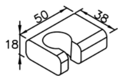
6909-9C-80CP Wall Bracket
