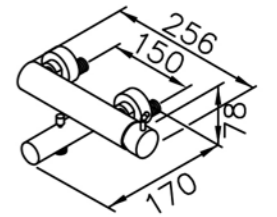
6768-94-80CP Bath / Shower Mixer Body
