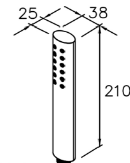
0922-9S-79CP Hand Shower (Plastic)
