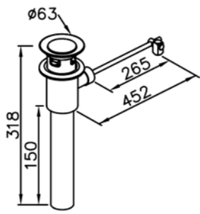
6502-A1-80CP Pop-Up W / Tail Tube & Overflow
