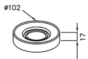
6502-CA-80CP Glass Basin Seat O.D 102*H17mm
