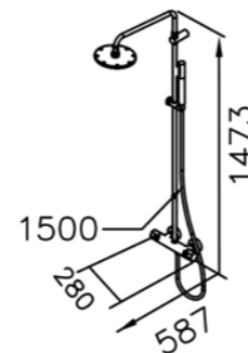
6771-TF-80CP Thermostatic Rainshower System
