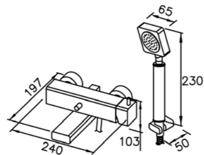
6909-94-81CP Bath / Shower Mixer W / Hand Shower W / Hose 150cm & Wall Bracket
