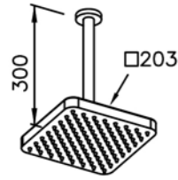
6909-AS-80CP Ceiling-Mounted 8" Showerhead ( Brass )
