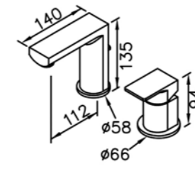
6790-X0-81CP Basin Faucet W / Lift Rod
