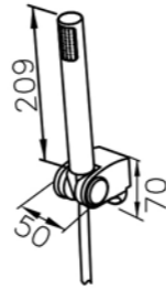
6759-9S-82CP Adjustable Wall Bracket W / Hand Shower W / Hose 150cm
