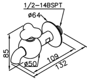
Bib Tap 6903-L0-80CP W / Brass-Sheet Flange 7903-L0-80CP W / Forged-Brass Flange
