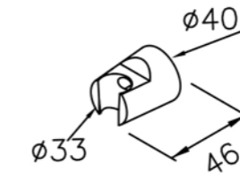
0758-9C-79CP Wall Bracket (Plastic)
