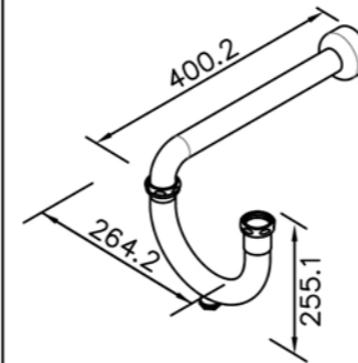
U-Trap W / Cleanout 6119-AU-80CP 1 1/2" 6119-BU-80CP 1 1/4"
