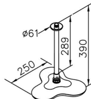
6903-AS-8007 Ceiling-Mounted Showerhead
