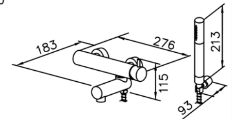
7771-94-81W1 Bath / Shower Mixer W / Hand Shower W / Hose 150cm W / Wall Bracket
