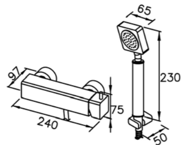
6909-93-81CP Shower Mixer W / Hand Shower W / Hose 150cm & Wall Bracket
