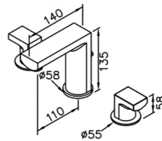
6790-91-81CP Two-Handle Lavatory Faucet W / Lift Rod
