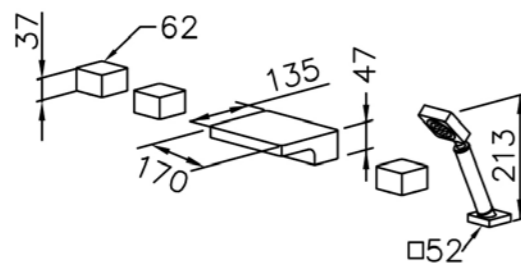
6909-M2-80CP Three-Handle Bathtub Faucet W / Hand Shower & Diverter
