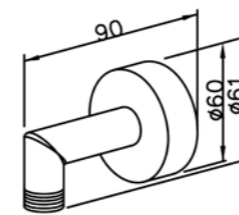
6880-AD-80CP Wall Supply G1/2
