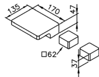
6909-M0-80CP Two-Handle Bathtub Faucet
