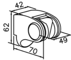
0759-9C-79CP Adjustable Wall Bracket ( Plastic )
