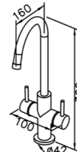
6796-96-80CP RO Faucet ( On Deck / Cold Only )
