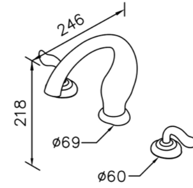
6781-91-80CP Two -Handle Lavatory Faucet
