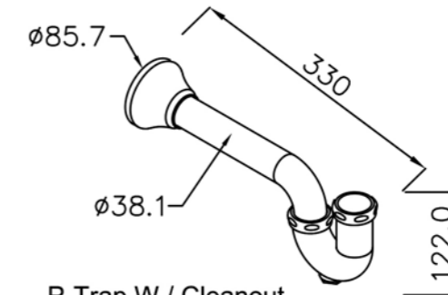
P-Trap W / Cleanout 6119-A3-80CP 1 1/2" 6119-B3-80CP 1 1/4"
