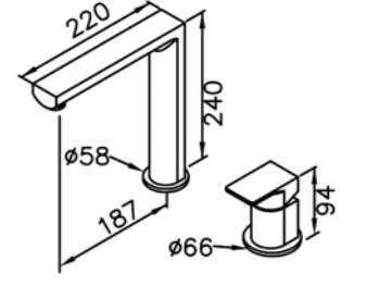
6790-X6-80CP Single-Handle Kitchen Faucet
