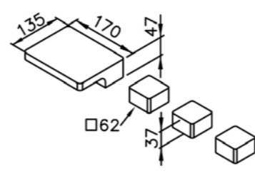
6909-M1-80CP Three-Handle Bathtub Faucet
