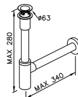
6502-A4-81CP Turn-Over With Overflow W / Tail Tube W / T-Trap(6502-T1-80CP)
