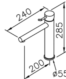
6768-96-80CP Kitchen Faucet Swivel Spout
