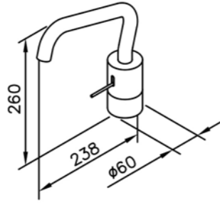
6777-96-80CP Kitchen Faucet
