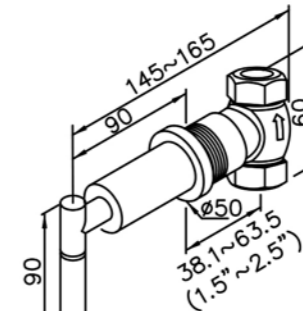
6880-VB-80CP Water Valve (Hot Only)
