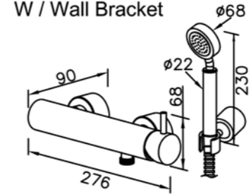
6771-94-81CP Bath / Shower Mixer W / Hand Shower W / Hose 150cm W / Wall Bracket
