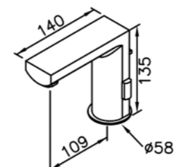
6790-N2-81CP Tip-Touch Basin Faucet W / Lift Rod
