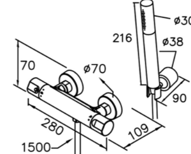
6771-T3-81CP Thermostatic Shower Mixer W / Hand Shower W / Hose 150cm W / Wall Bracket
