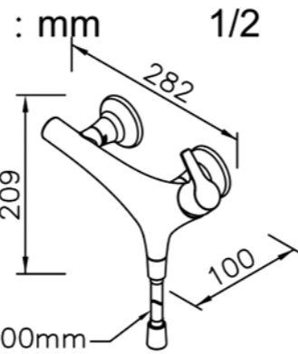
6927-93-85CP Shower Mixer Body W / Hose 150 cm
