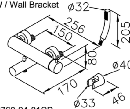
6768-94-81CP Bath / Shower Mixer W / Hand Shower W / Hose 150cm W / Wall Bracket
