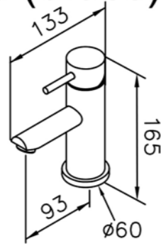
6757-91-80CP Basin Faucet
