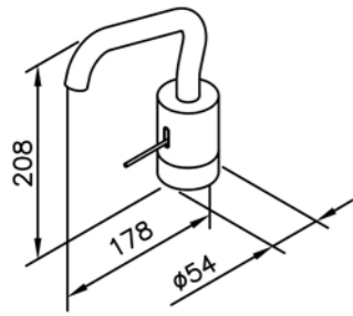
6777-90-80CP Basin Faucet
