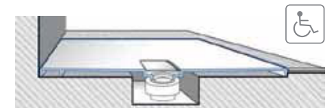
FLUSH-FIT INSTALLATION
