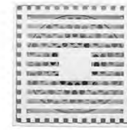
0303-64-79CW Floor Drain Brass Size 100*100 mm Height 51 mm Seal Type Self Seal Brass Flow Rate \geq 15L/Min Outlet OD 40 mm Drain Core 0303-A1-7900
