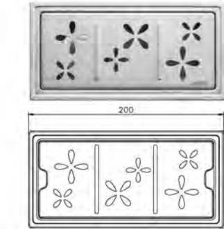
0305-01-79S1 Floor Drain SUS 304 Size 200*100 mm Height 59 mm Seal Type Self Seal Brass Flow Rate ≥18L/Min Outlet OD 42mm Drain Core 0305-A1-7900
