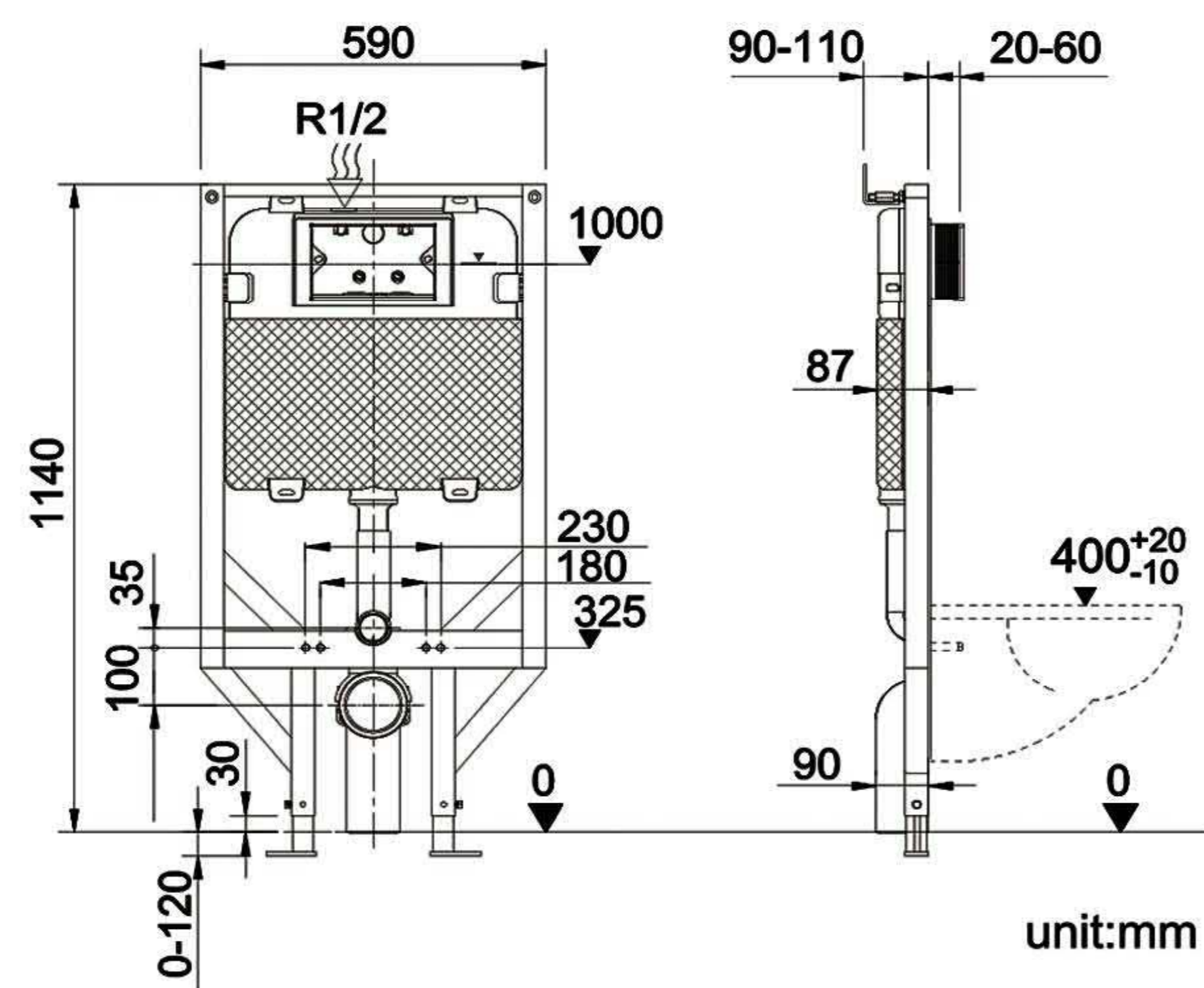
6373-01-8000 Concealed Cistern
