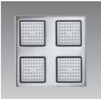
WaterTile Rain overhead showering panel with 4 individually adjustable 54-nozzle WaterTile sprayheads 8030W
