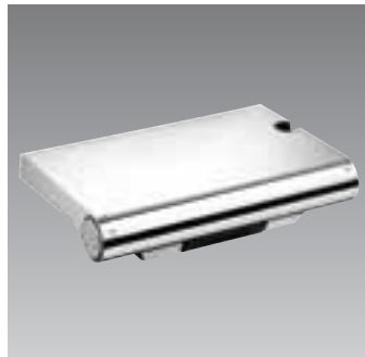
Thermostatic 2-handle 2-hole wall-mount bath/shower mixer incl. wall mount mixing valve Diverter on flow handle Integral handshower holder Waterfall effect 9113D
